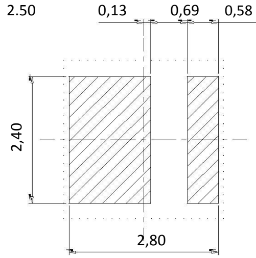
Soldering patterns
