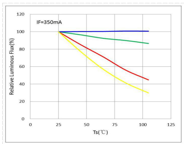
Fig 5. Ambient Temperature vs. Relative Luminous flux ( I_F=350\text{mA} )
